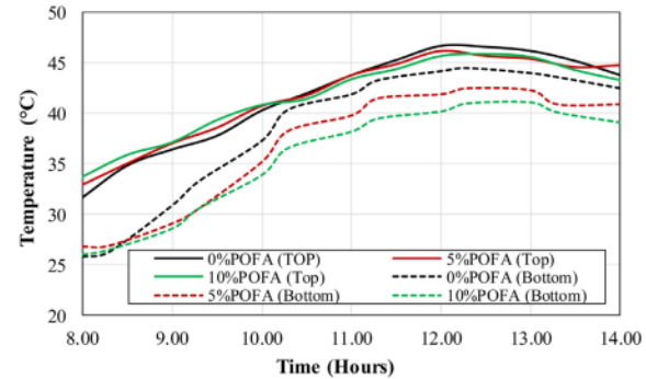
Fig. 11. Variation in the top and bottom surface temperatures of bricks exposed to direct sunlight over time.
