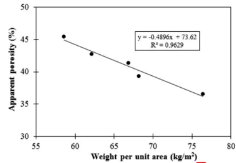
Fig. 8. Relationship between the apparent porosity and the weight per unit area of brick specimens.
