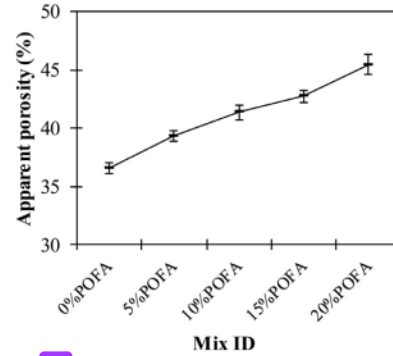
Fig. 7. Apparent porosity of brick specimens.
