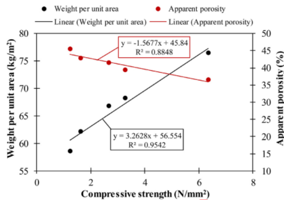
Fig. 10. Relationship between compressive strength, weight per unit area, and apparent porosity of the POFA brick specimens.
