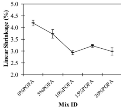
Fig. 5. Brick linear shrinkage.
