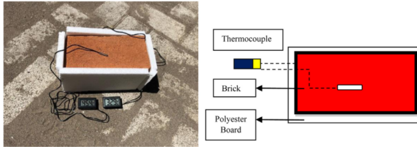
Fig. 4. Experimental setup to evaluate the thermal performance of brick specimens.
