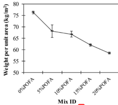
Fig. 6. Weight per unit area of brick specimens.
