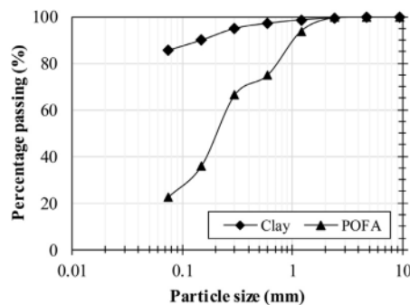
Fig. 3. Particle size distribution of clay and POFA.
