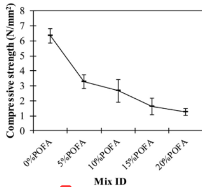
Fig. 9. Compressive strength of bricks.
