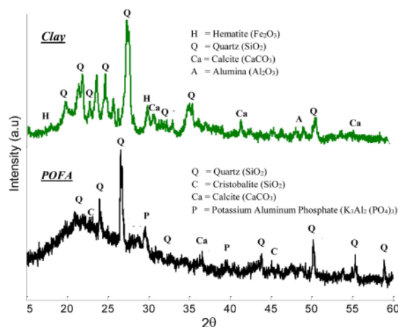
Fig. 1. XRD patterns of clay and POFA.
